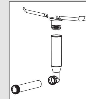
Water flow is 2.1 ltrs. by seconds for perfect pan rinsing. Large flush volume can be increased to 2.5 ltrs.
